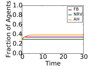
Figure 5: Contagion spread (in terms of fraction of agents affected) via classic threshold diffusion [5] in the three networks where p_p = 1.0 , and for each network, 30% of the populations are seeded with the contagion. Thresholds for the FB, NRV, and AH networks are, respectively, 9, 12, and 4.
